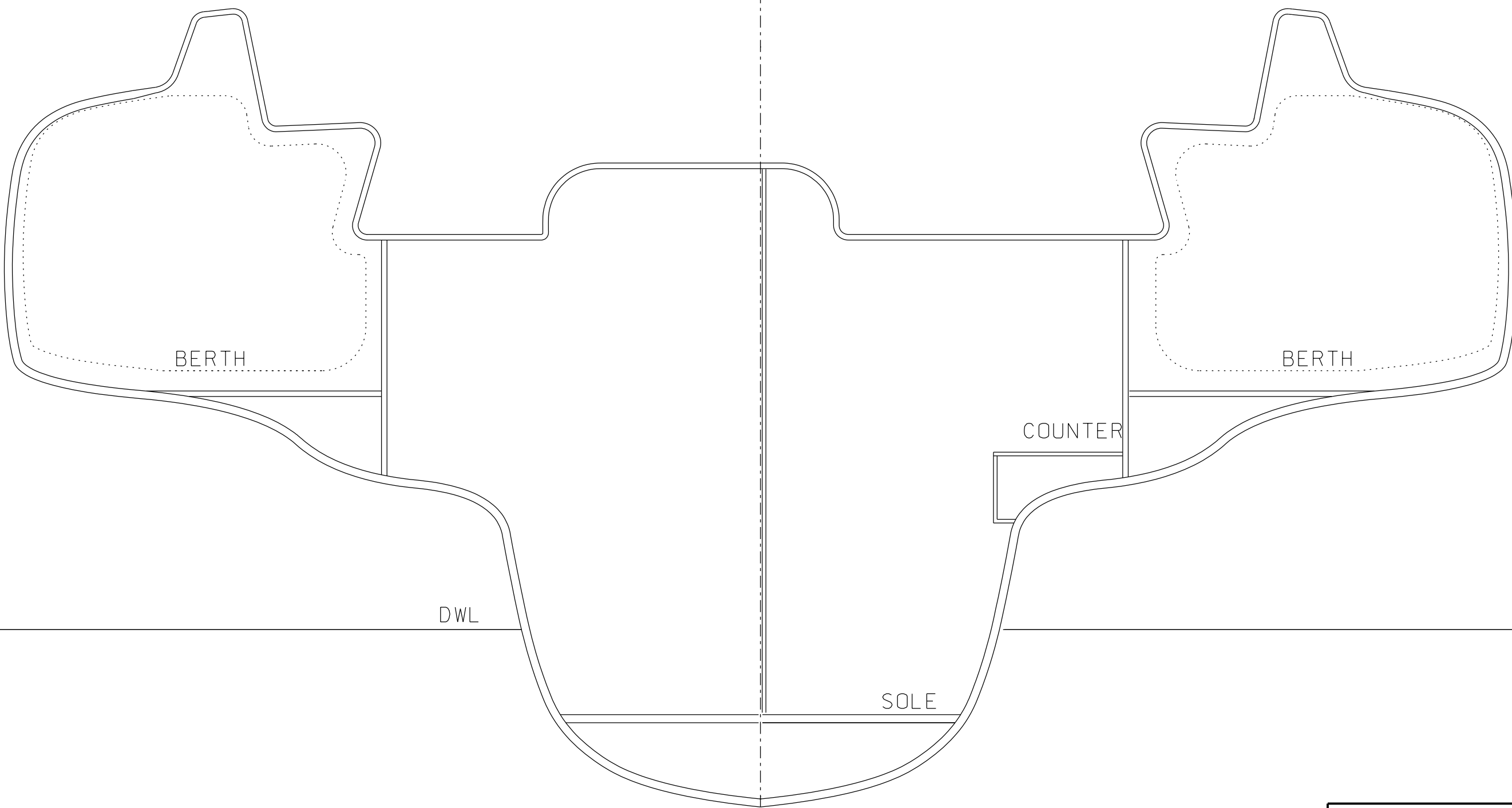
DETAIL SECTION @ STATION #21
