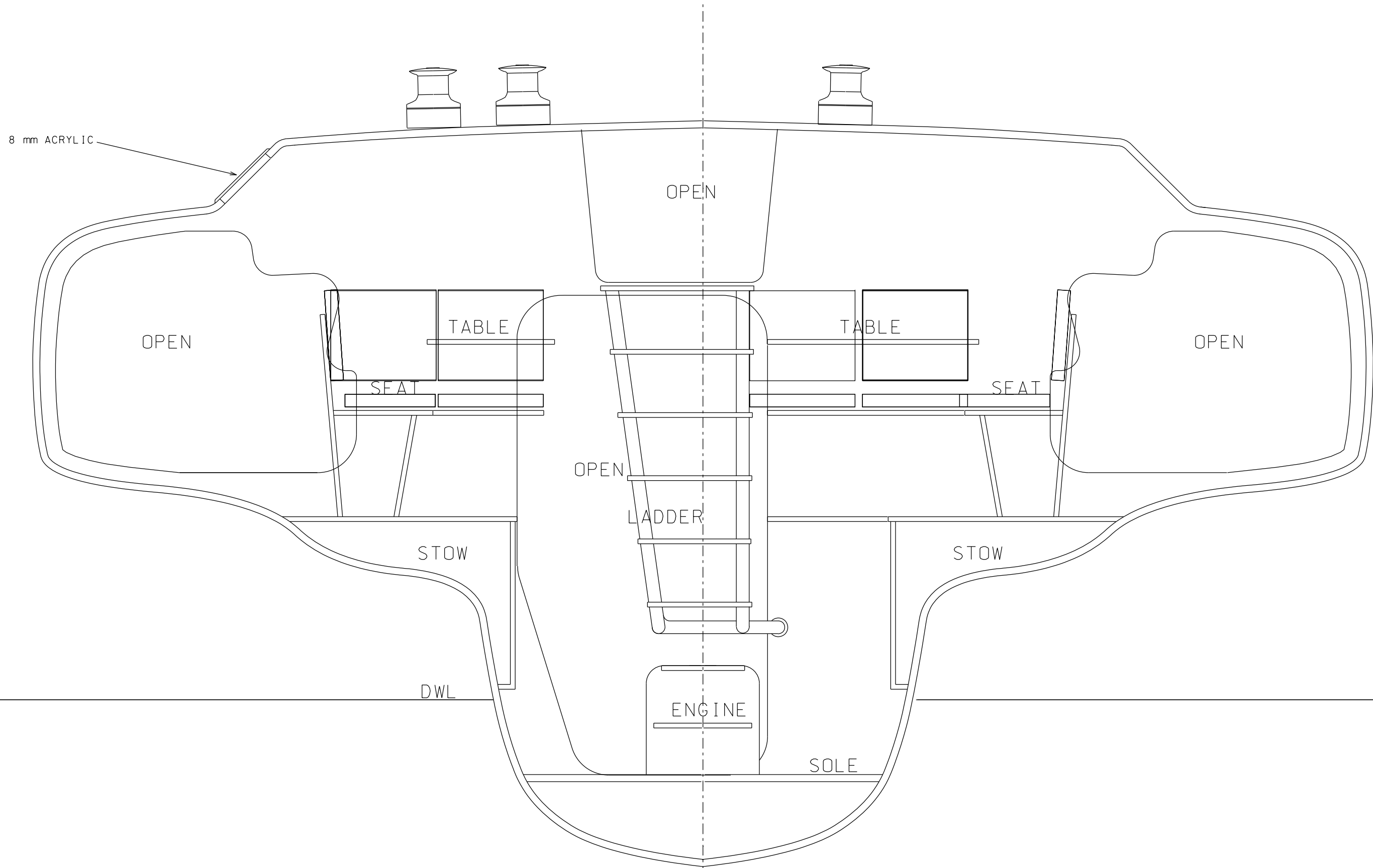
DETAIL SECTION @ STATION #18
