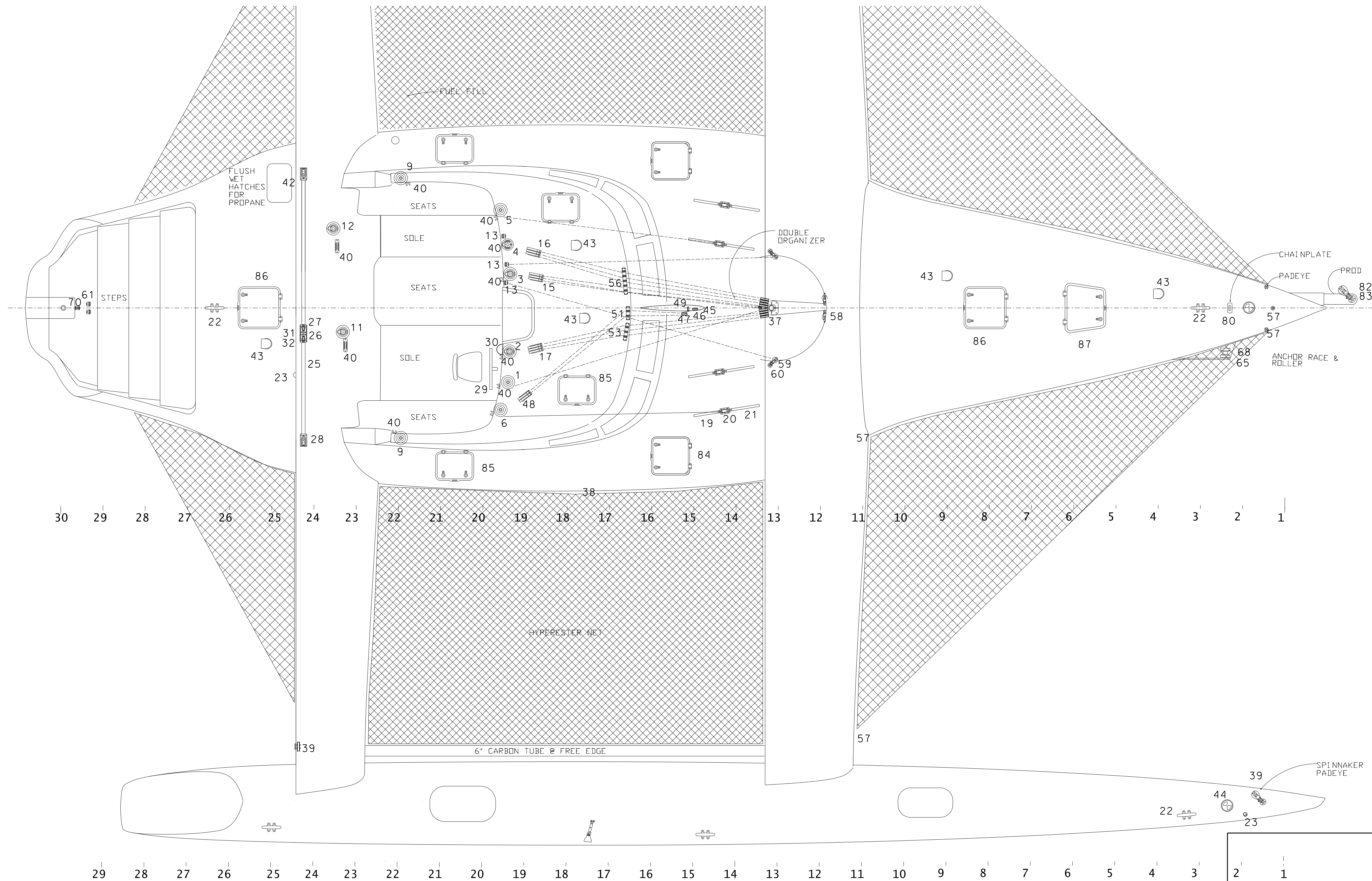
DECK HARDWARE SCALE 1:25
